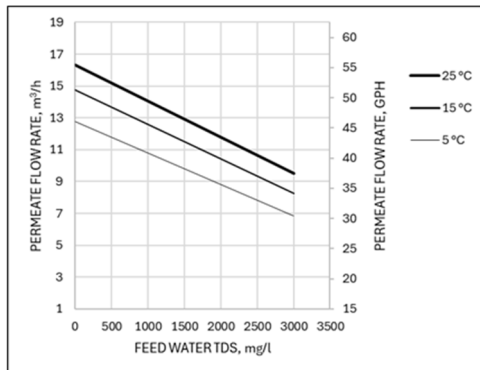
Ecosoft MO9 flow rate chart
