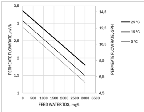
Ecosoft MO2 flow rate chart
