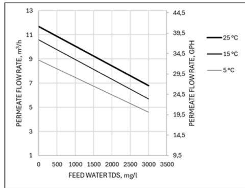
Ecosoft MO6 flow rate chart
