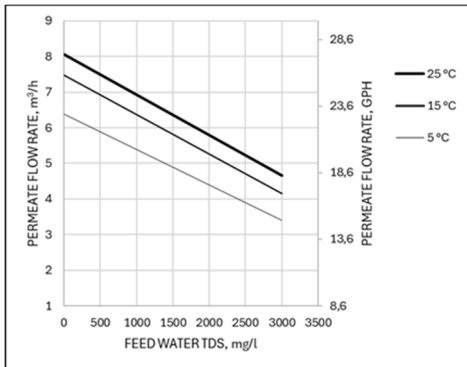
Ecosoft MO4 flow rate chart
