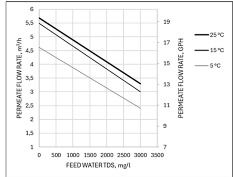
Ecosoft MO3 flow rate chart
