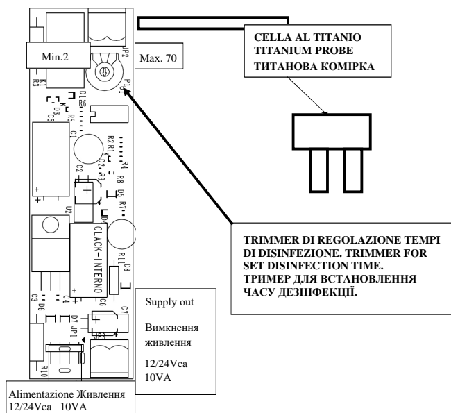
Electrical diagram
